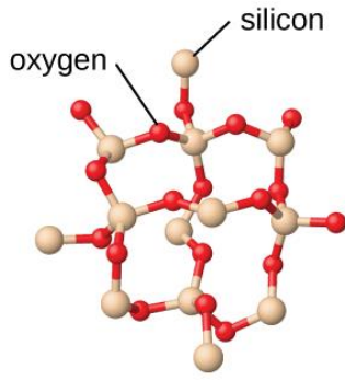
silicon dioxide
