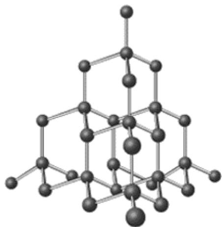
(a) Diamond
