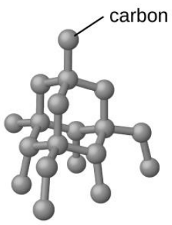
diamond
