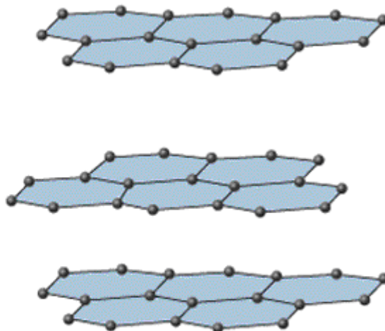
(b) Graphite
